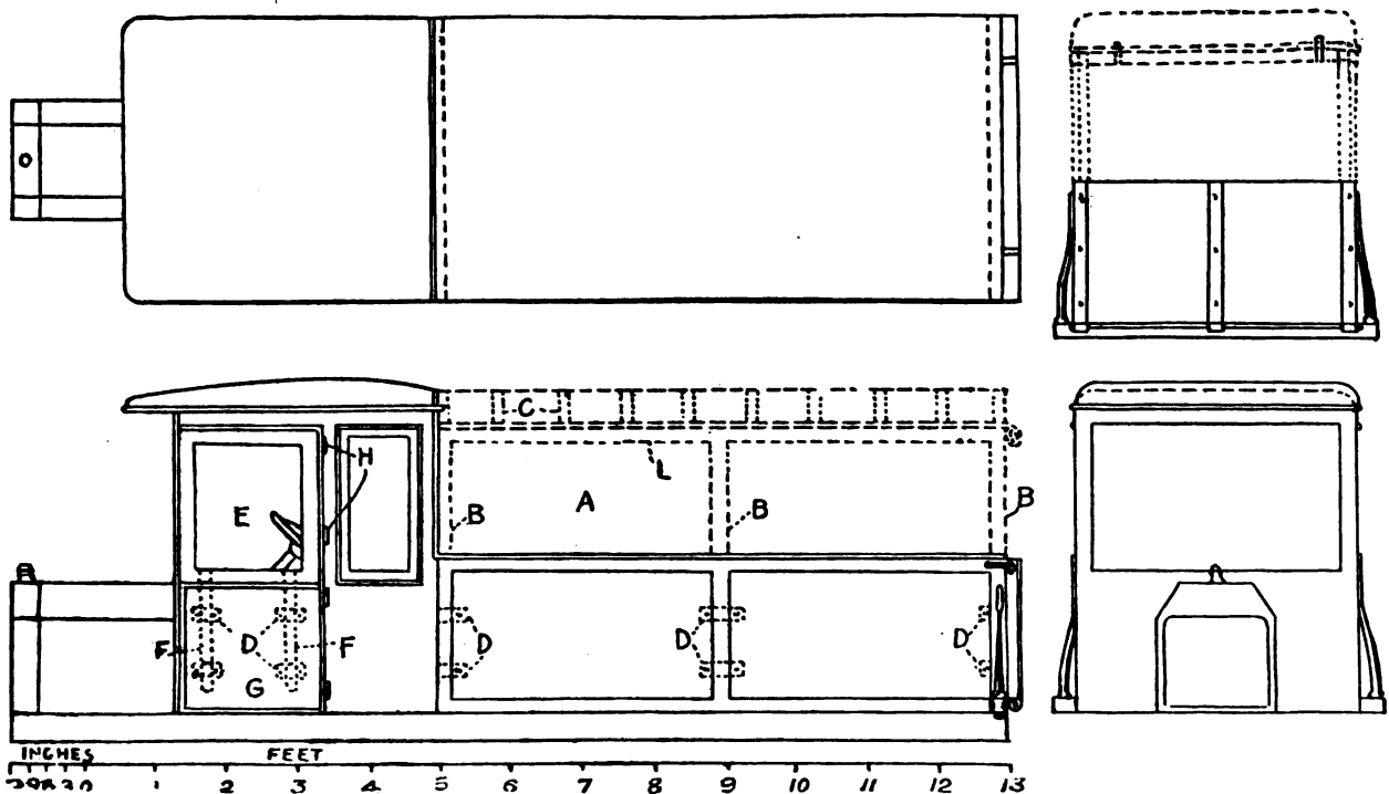
Fig. 2—Working draft of top and cover and driver's cab for open type of commercial car
